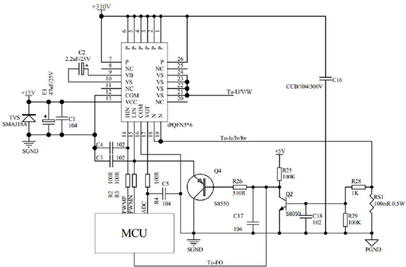
Fig.8 Typical Application Connection NSH505PQ
