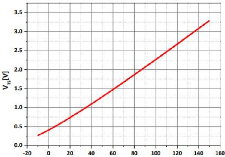
Fig. 4 Curves of HVIC Temperature detection—voltage curve
