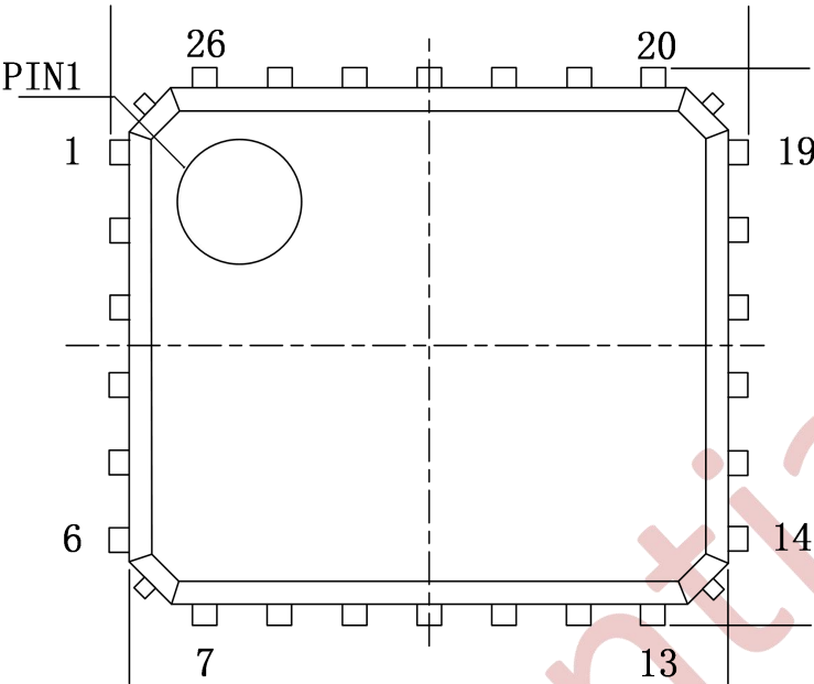
Fig2 Footprint Description
