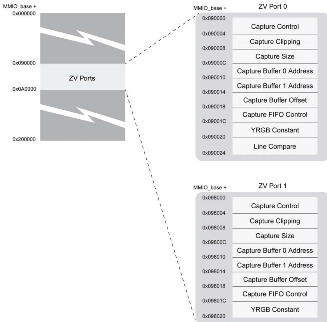
Figure 30: ZV Port Register Space
