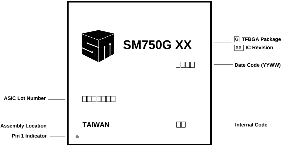
Figure 39: SM750 0MB IC Marking (Commercial version)
