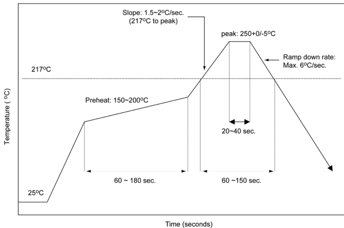
Figure 35: Temperature Profile
