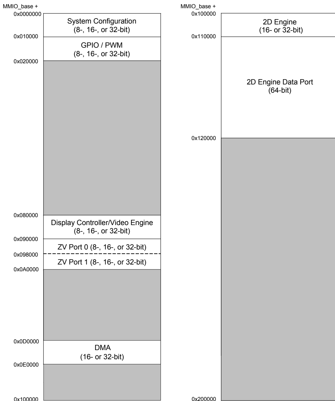
Figure 11: MMIO Space
