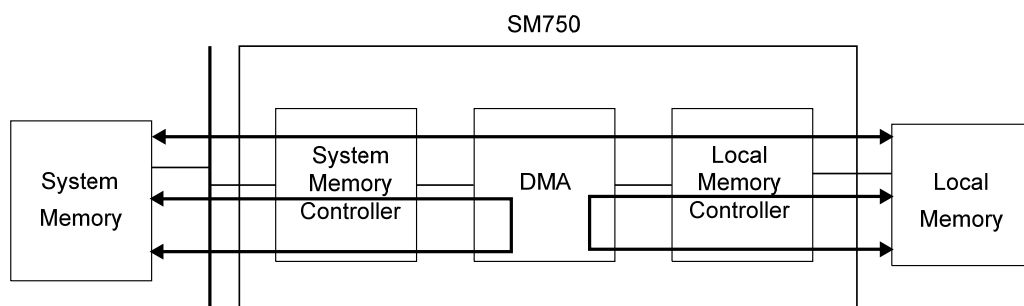
Figure 32: DMA Channel 1
