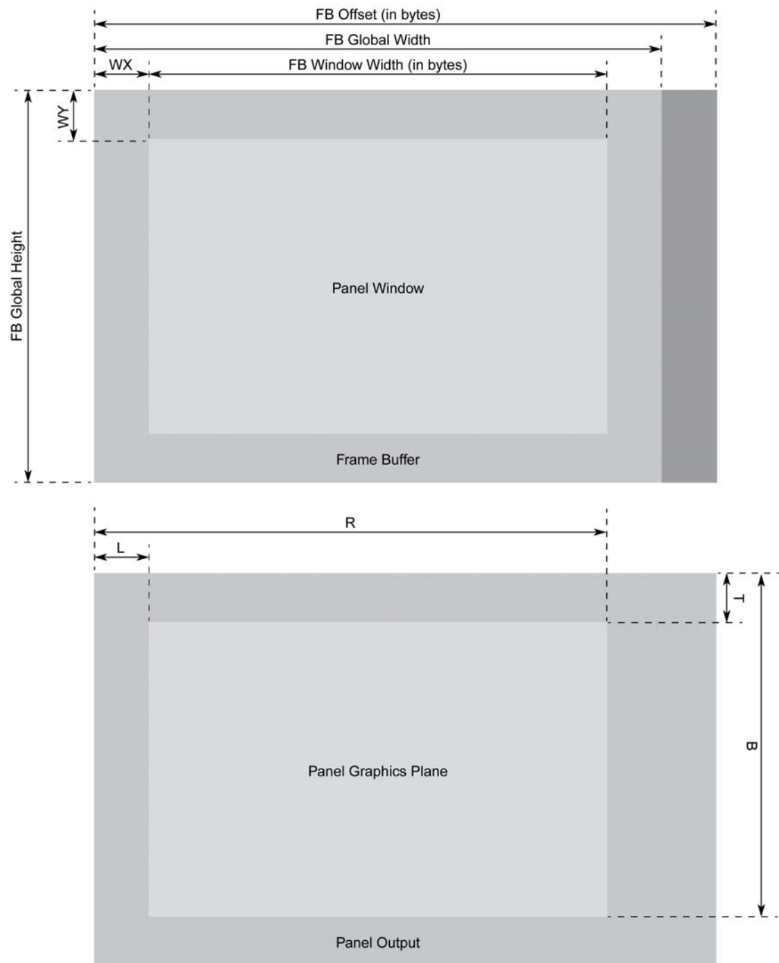
Figure 19: Video Windowing
