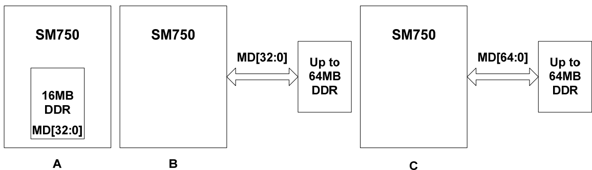
Figure 5: Memory Setups
