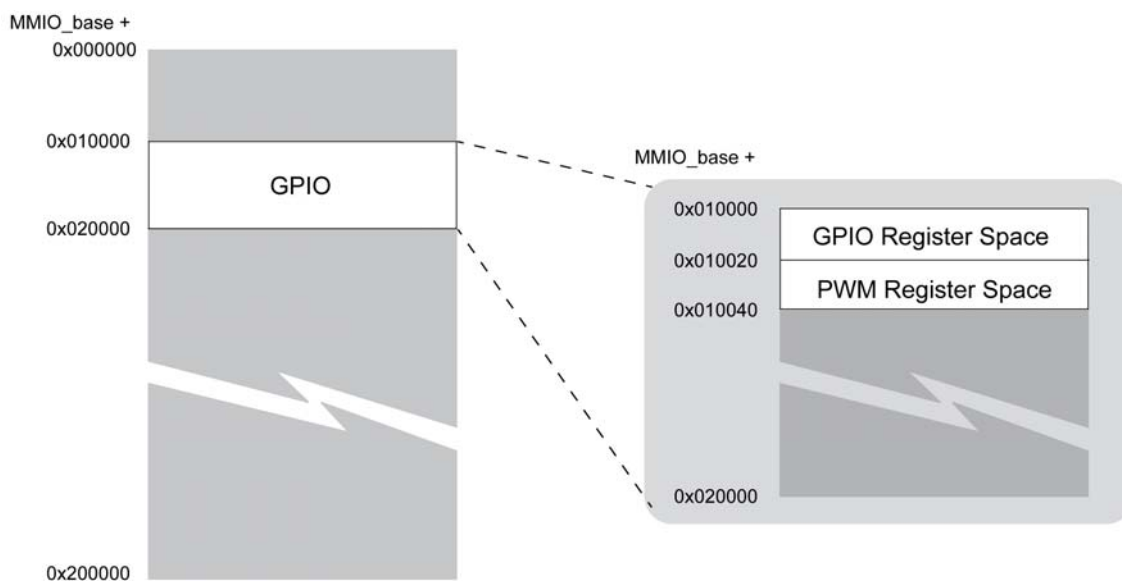
Figure 27: GPIO Register Space
