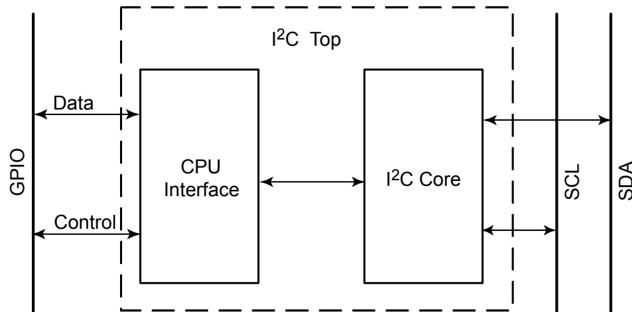
Figure 29: I 2 C Interface block diagram
