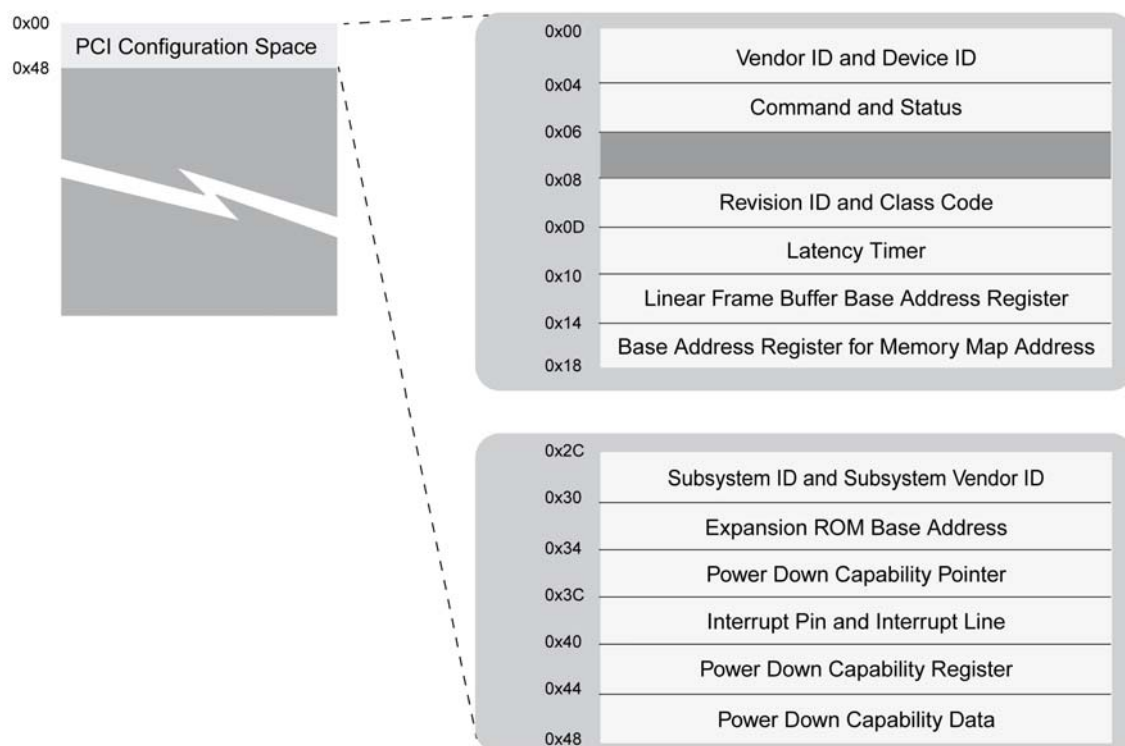
Figure 12: PCI Configuration Register Space
