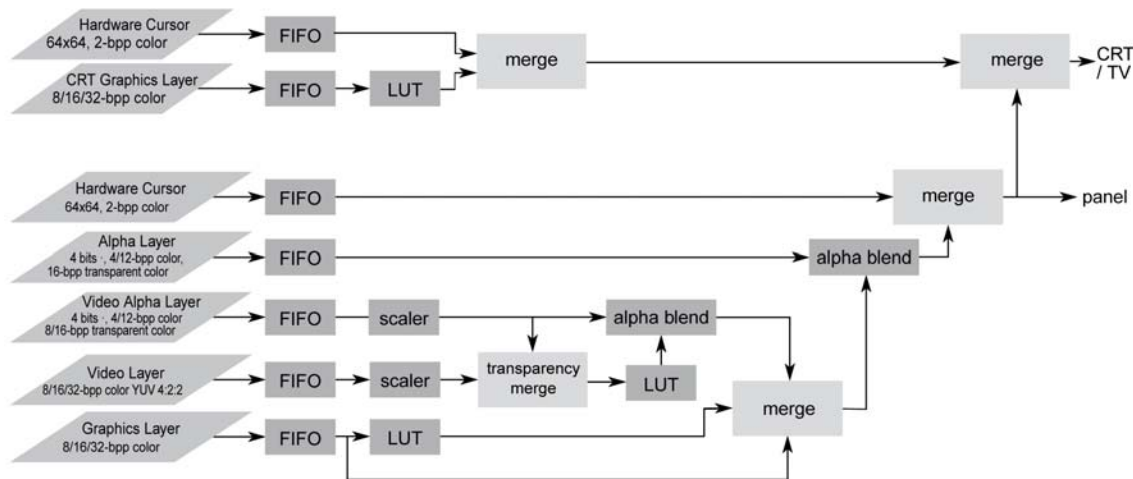
Figure 17: Video Layers
