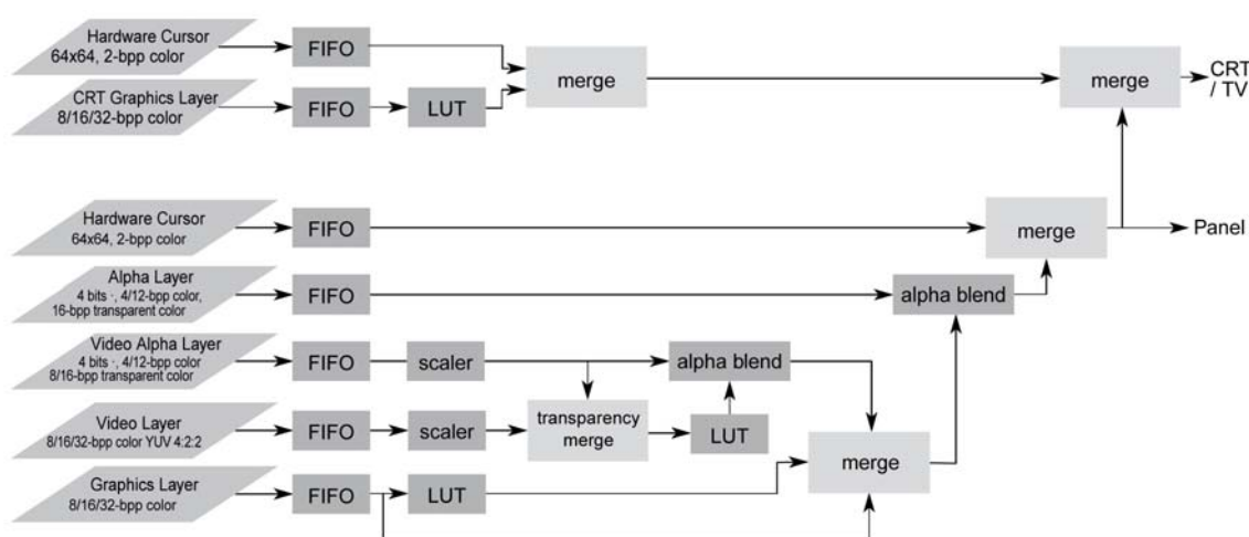
Figure 7: Video Layers and Data Processing
