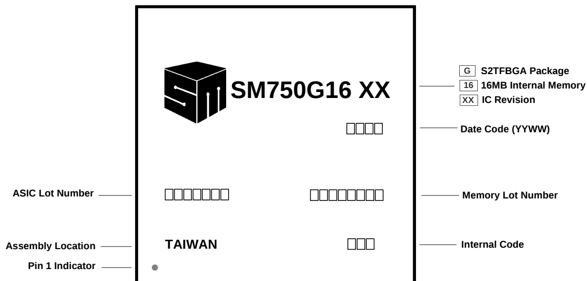
Figure 40: SM750 16MB IC Marking (Commercial version)
