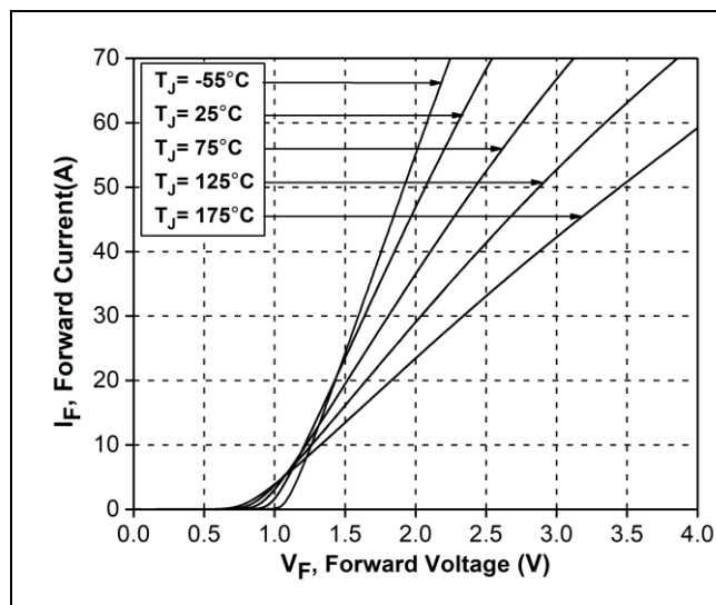
Figure 1. Forward Characteristics
