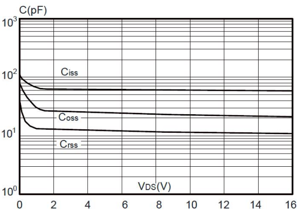
Figure 5: Capacitance Characteristics
