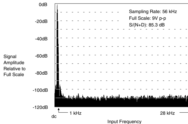
Figure 21. CS5014 FFT plot with 1 kHz Full Scale Input
