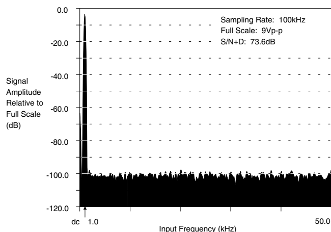
Figure 18. Plot of CS5012A with 1 kHz Full Scale Input
