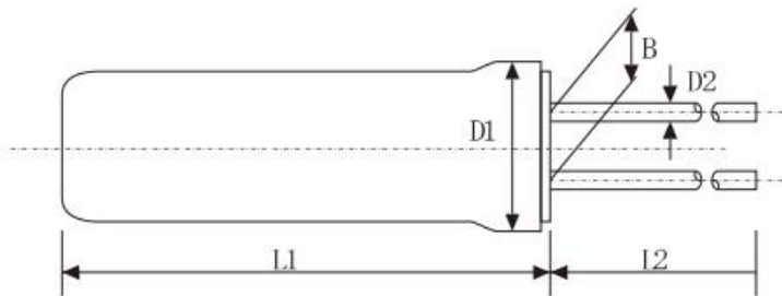
Package Size – Dimensions (Unit: mm)
