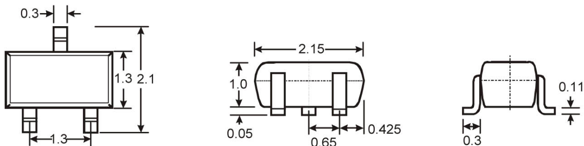
Figure 3. MDD7630-323 Outline Drawing
