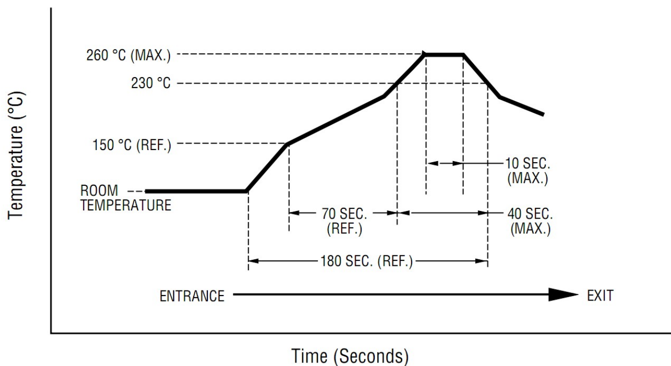
Figure 4. MDD7630-323 Thermal Reflow Profile
