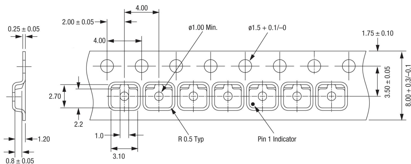
Figure 5. MDD7630-323 Packaging Information
