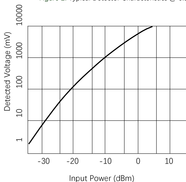
Figure 2. Typical Detector Characteristics @ 0.9
