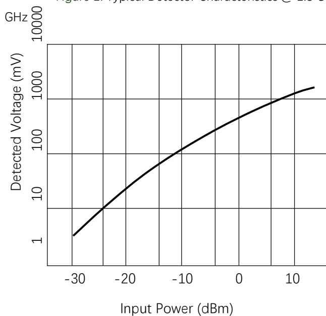
Figure 1. Typical Detector Characteristics @ 1.8 GHz
