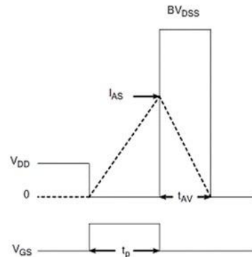
Figure 19 Unclamped Inductive Switching Waveform
