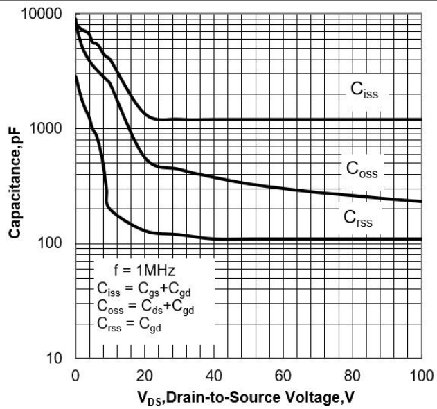
Figure 10 Capacitance Characteristics
