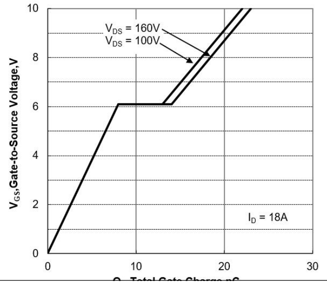
Figure 11 Gate Charge Characteristics
