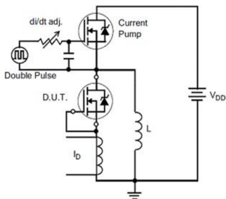
Figure 18 Unclamped Inductive Switching Test Circuit
