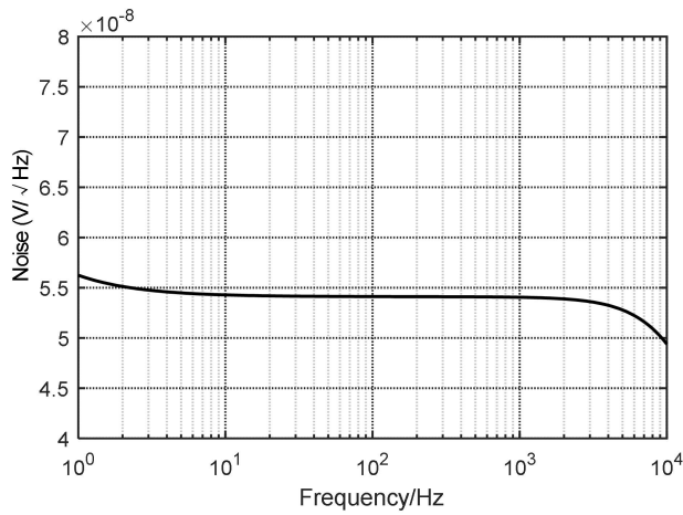
Fig.8-3. Noise Response
