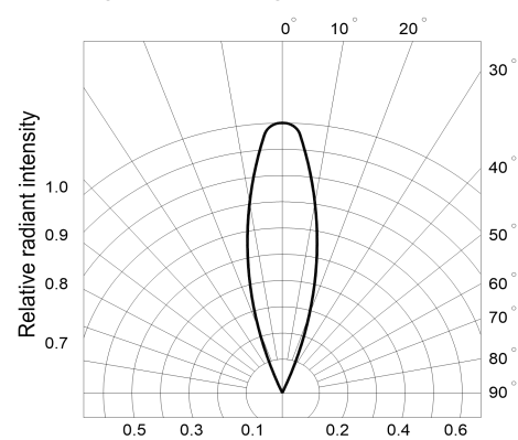
Fig.6 Radiation diagram
