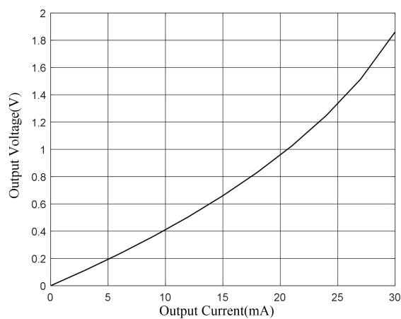
Fig.8-3. Output Voltage vs Output Current
