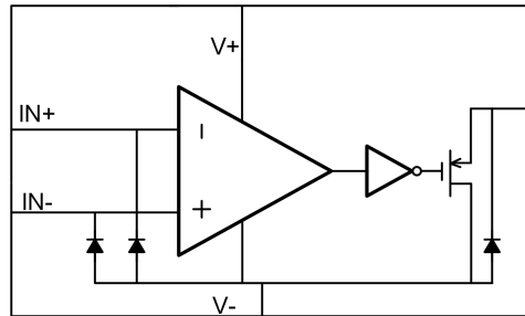
Fig.9-1. Functional Block Diagram
