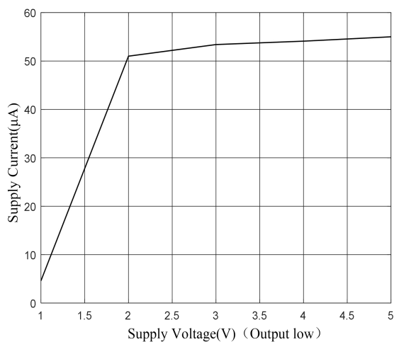
Fig.8-1. Supply Current vs Supply Voltage Output Low
