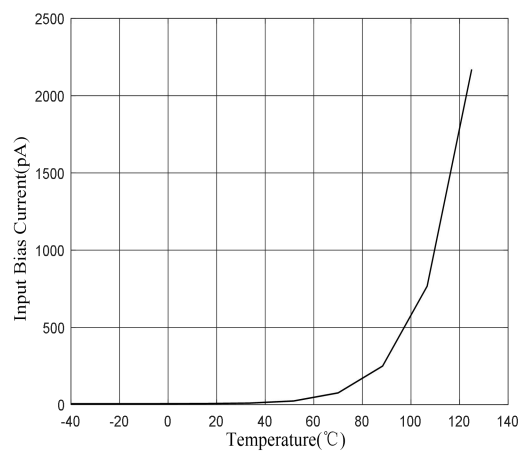
Fig.8-4. Input bias current vs temperature
