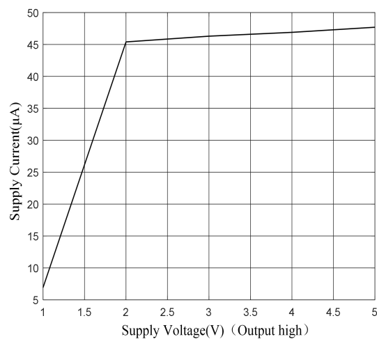
Fig.8-2. Supply Current vs Supply Voltage Output High
