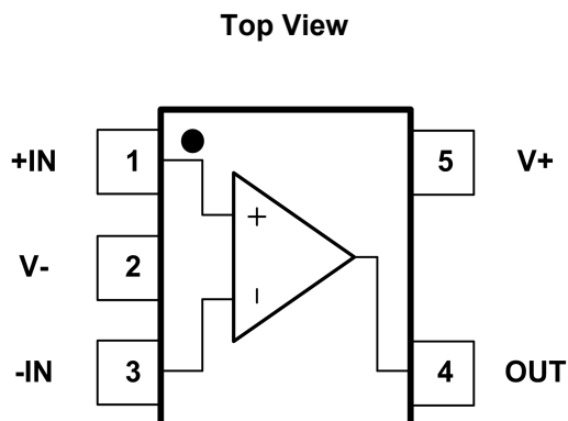
Fig.5-1. GT331: S5 (SOT23-5) Package
