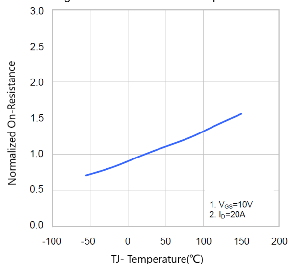
Figure 6. Rds(on)-Junction Temperature
