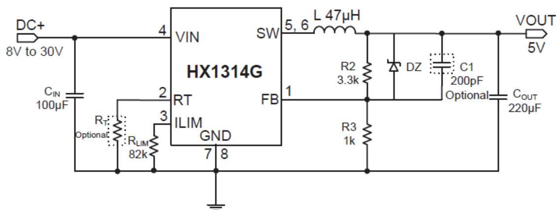
Application1: No Output Cable Resistance Compensation (Note 1)
