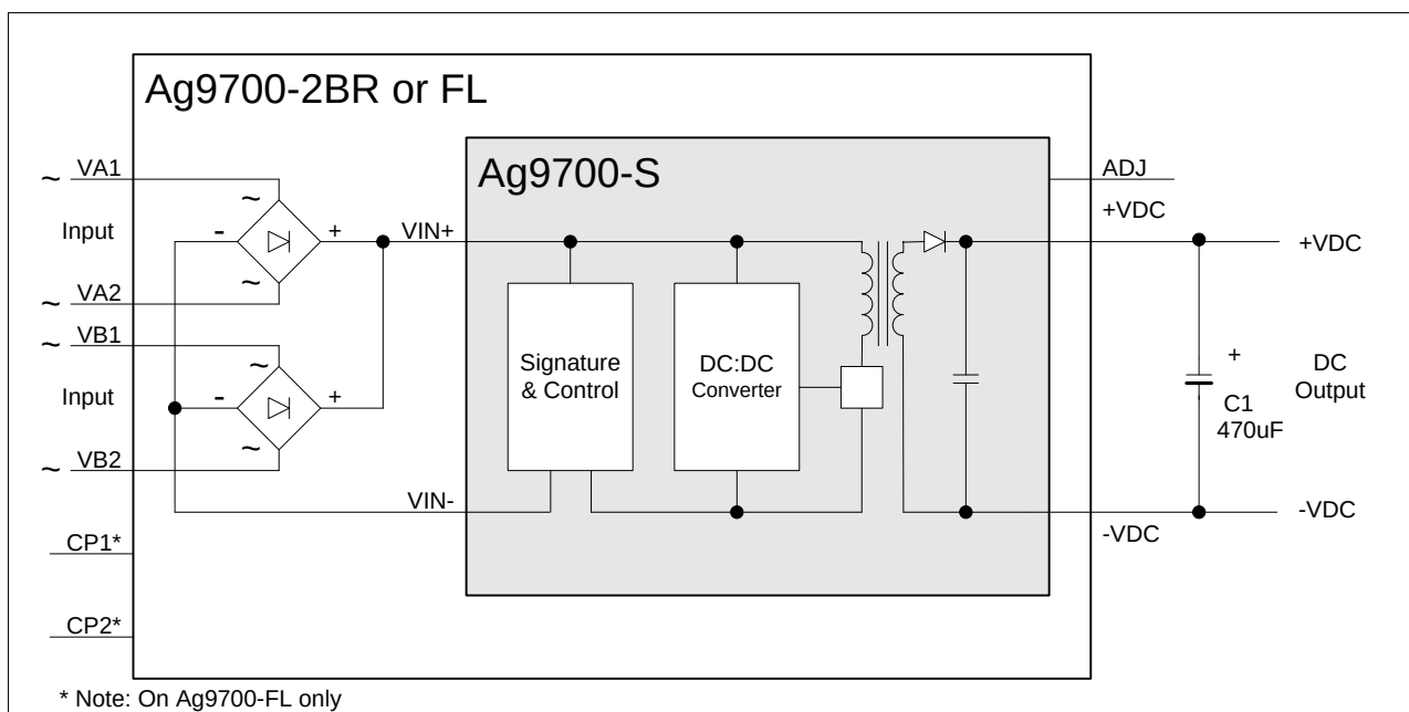
Figure 1: Block Diagram
