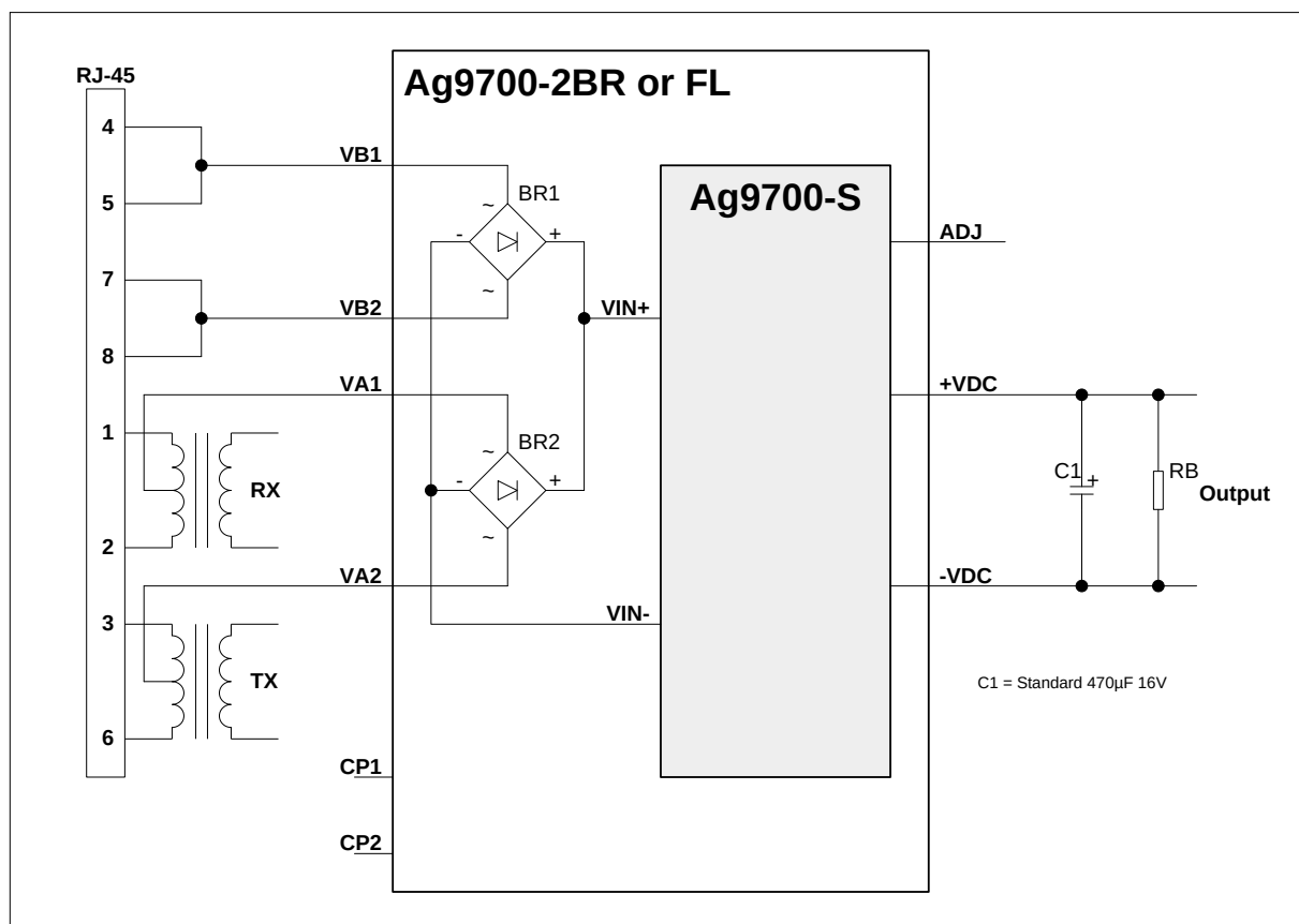
Figure 6: Basic Connection Diagram
