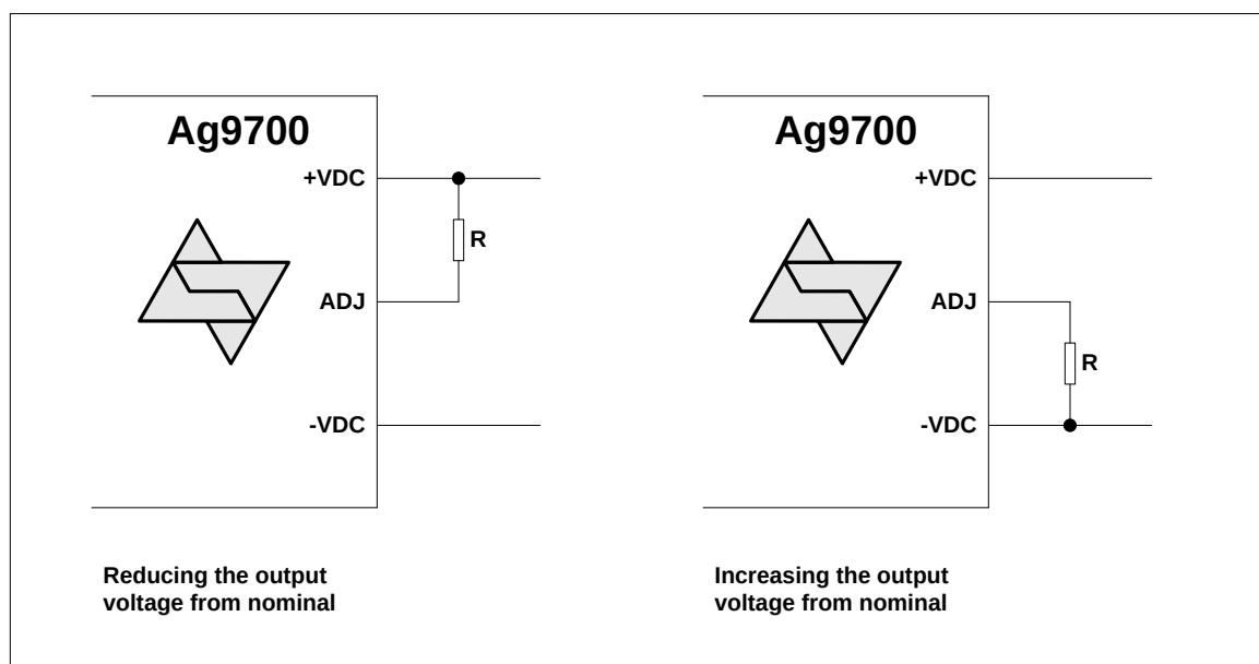
Figure 5: Output Adjustment
