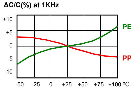
Temperature Characteristics
