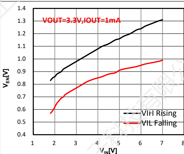
Figure 6. V_{EN} vs V_{IN}
