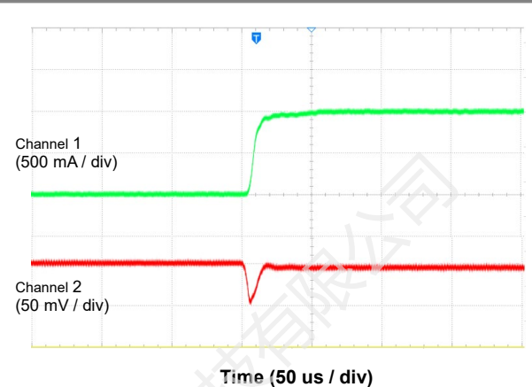
Channel 1 = I_{OUT} , channel 2 = V_{OUT} , V_{IN} = 1.8V, V_{OUT} = 0.8V Figure 17. Load Transient (1 mA to 1000 mA)
