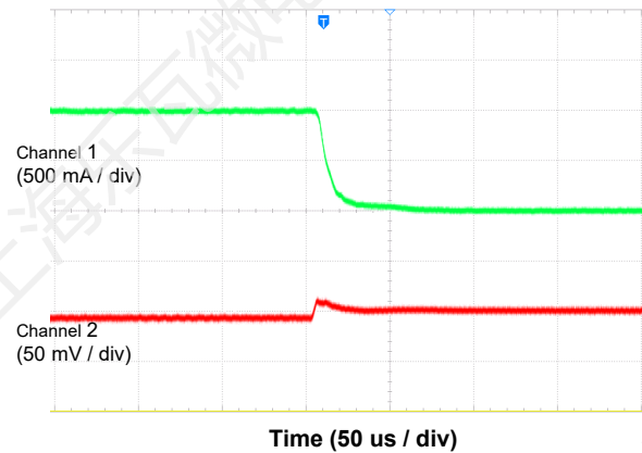
Figure 20. Load Transient (1000 mA to 1 mA)
