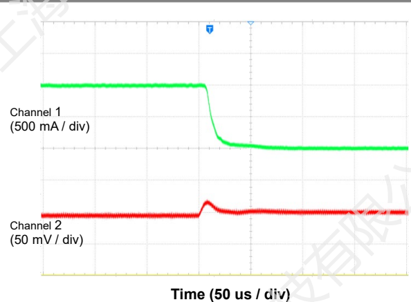
Channel 1 = I_{OUT} , channel 2 = V_{OUT} , V_{IN} = 1.8V, V_{OUT} = 0.8V Figure 18. Load Transient (1000 mA to 1 mA)
