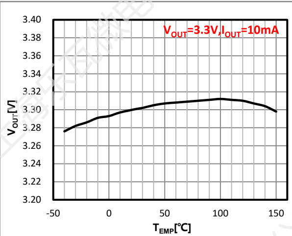
Figure 2. V_{OUT} vs Temperature
