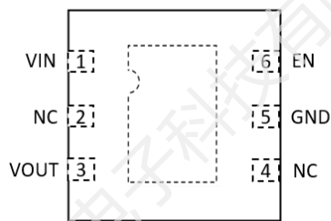
DFN2x2-6L
