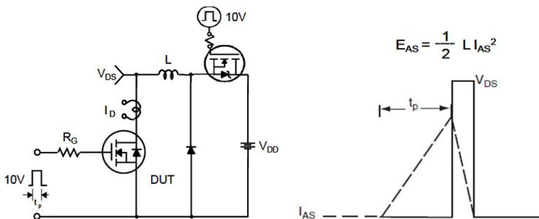
Unclamped Inductive Switching Test Circuit & Waveforms
