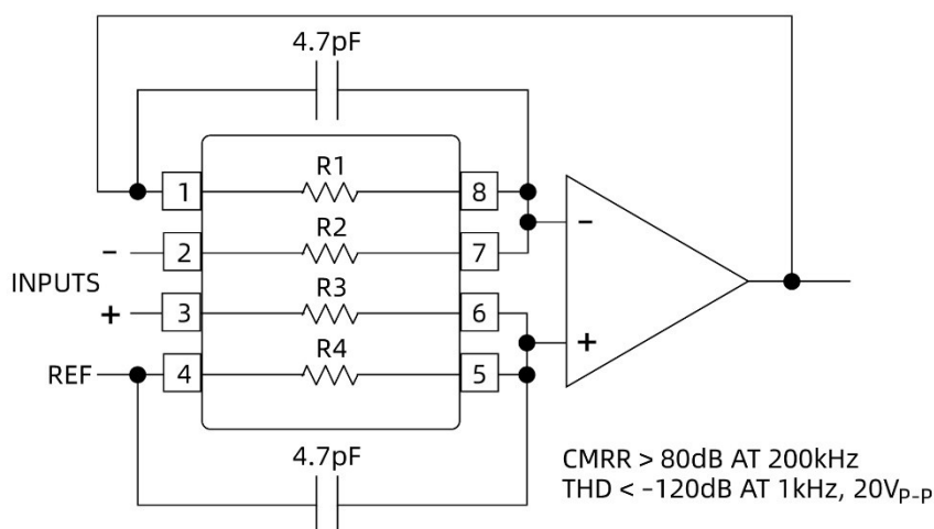
Figure 1. Difference Amplifier
