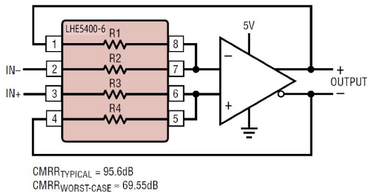
Figure 5. Gain of 5, Fully-Differential Amplifier
