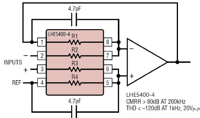
Figure 4. Difference Amplifier
