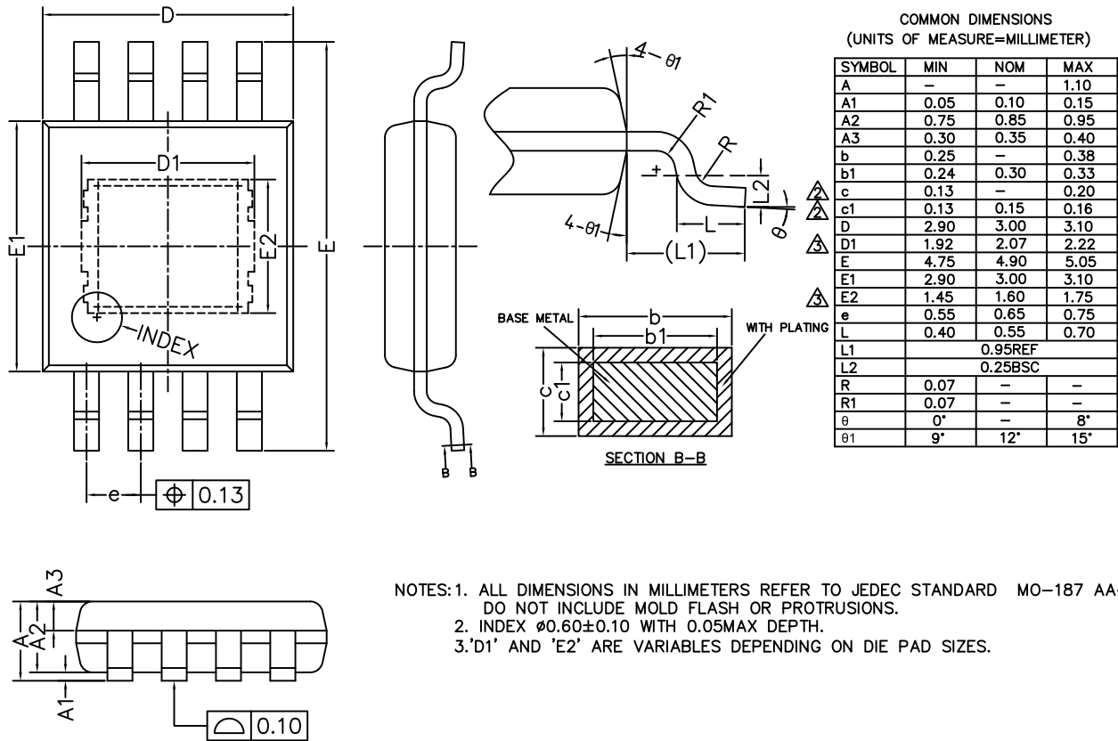
Figure 6. Package Description
