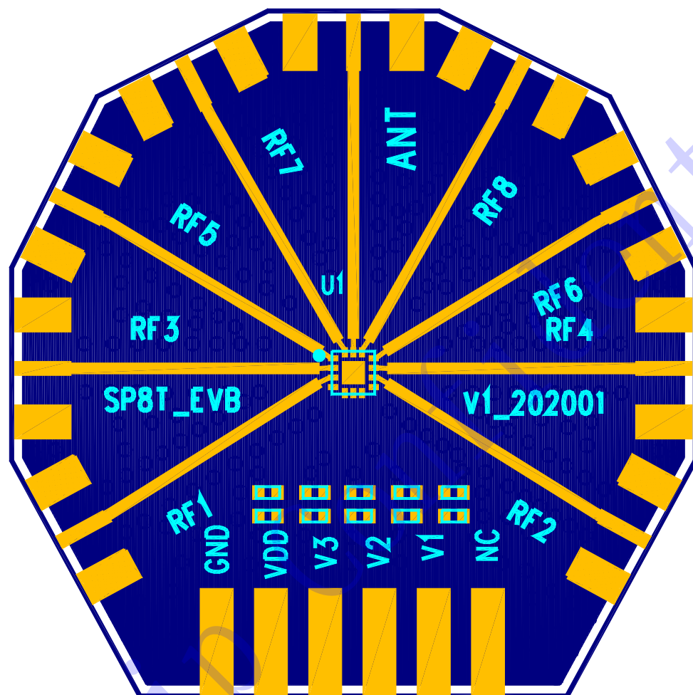
Figure 4 Evaluation Board Assembly Diagram
