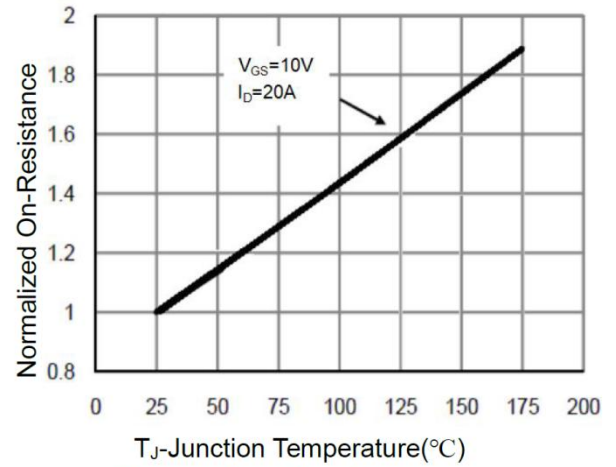
Rdson-Junction Temperature
