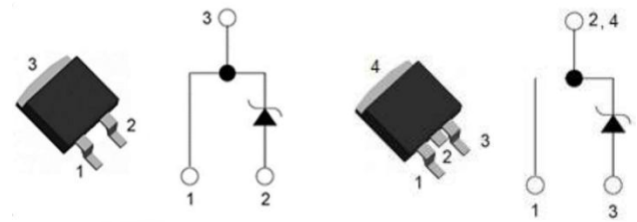
TO-252/DPAK
