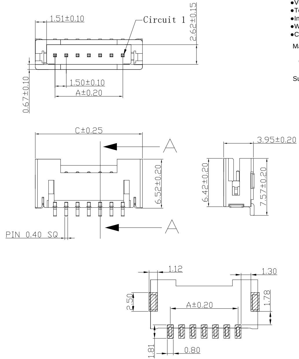
SECTION A—A
