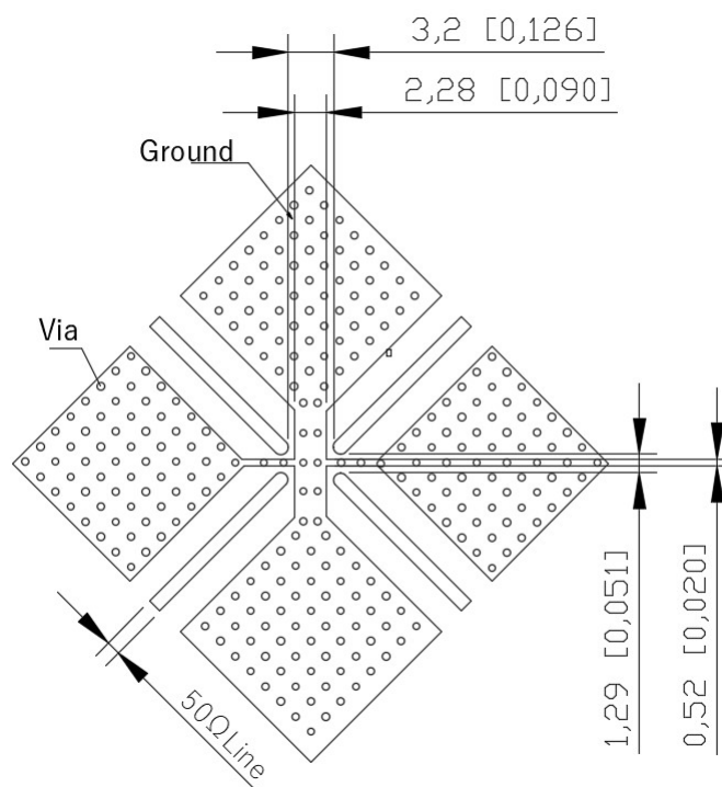
Figure 9. MHC09X02 Recommended PCB Layout
