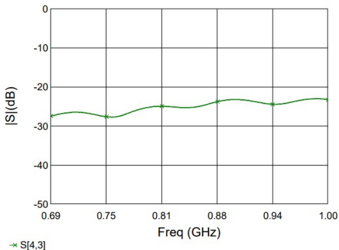
Figure 7. MHC09X02 Isolation
