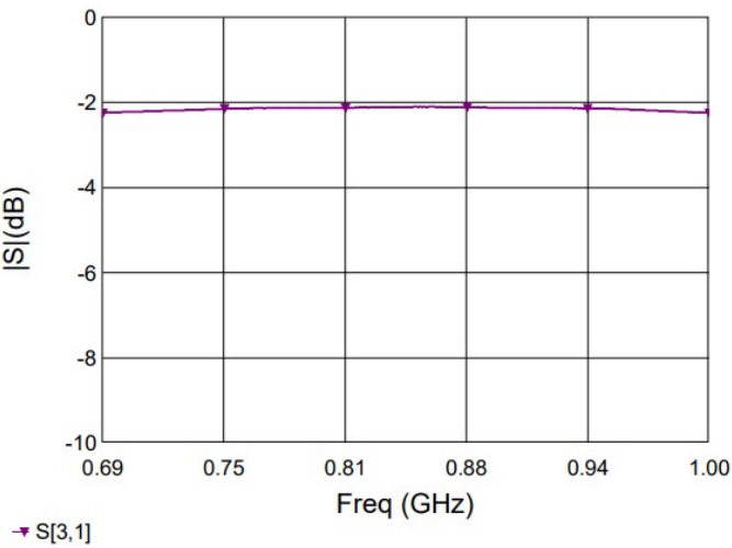
Figure 3. MHC09X02 Coupling
