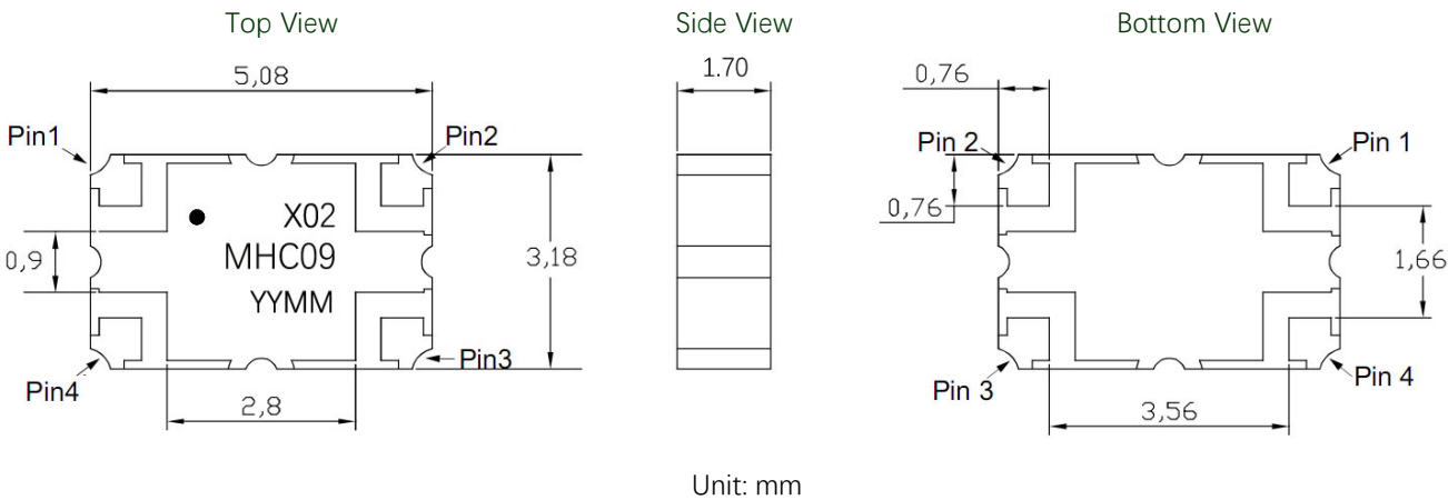
Figure 2. MHC09X02 Outline Drawing
