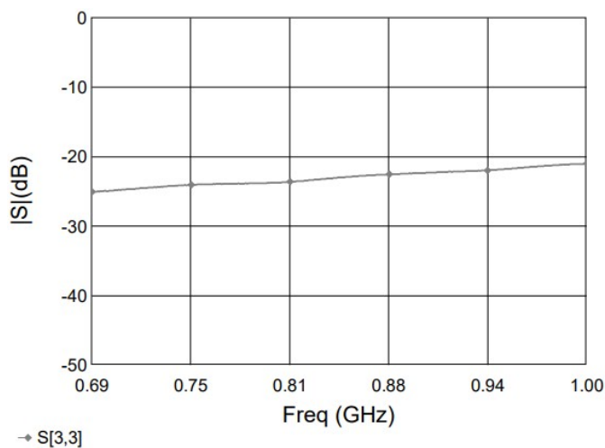
Figure 5. MHC09X02 Return Loss (S33)
