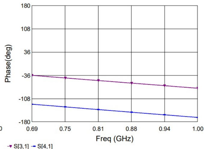
Figure 8. MHC09X02 Phase
