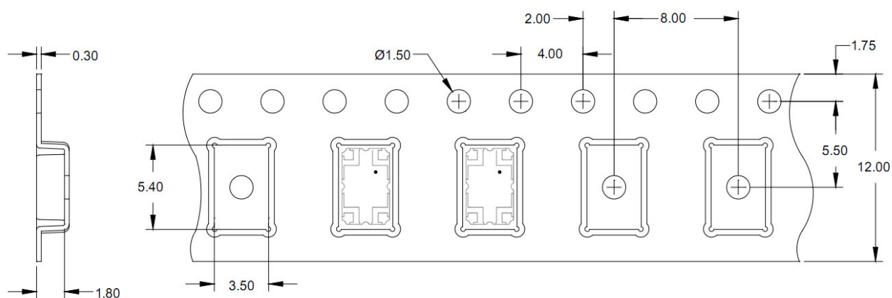
Figure 11. MHC09X02 Packaging Information
