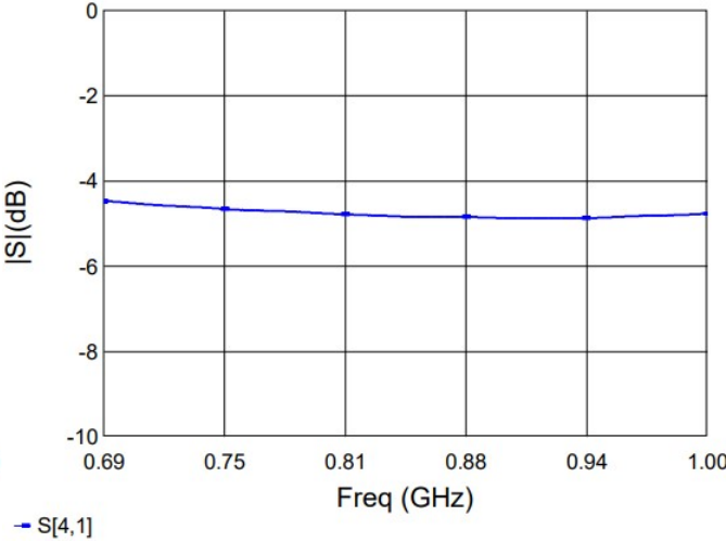
Figure 4. MHC09X02 Transmission
