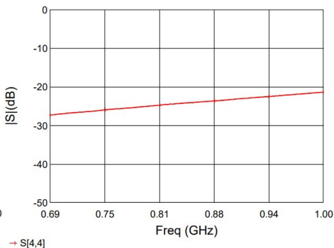
Figure 6. MHC09X02 Return Loss (S44)
