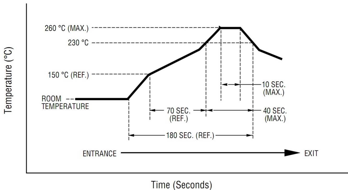
Figure 10. MHC09X02 Thermal Reflow Profile
