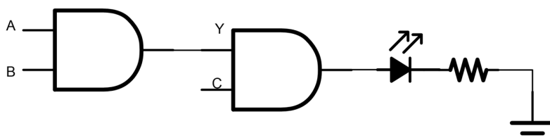
Fig.11-1.Three Input AND Gate Implementation and Driving LED
