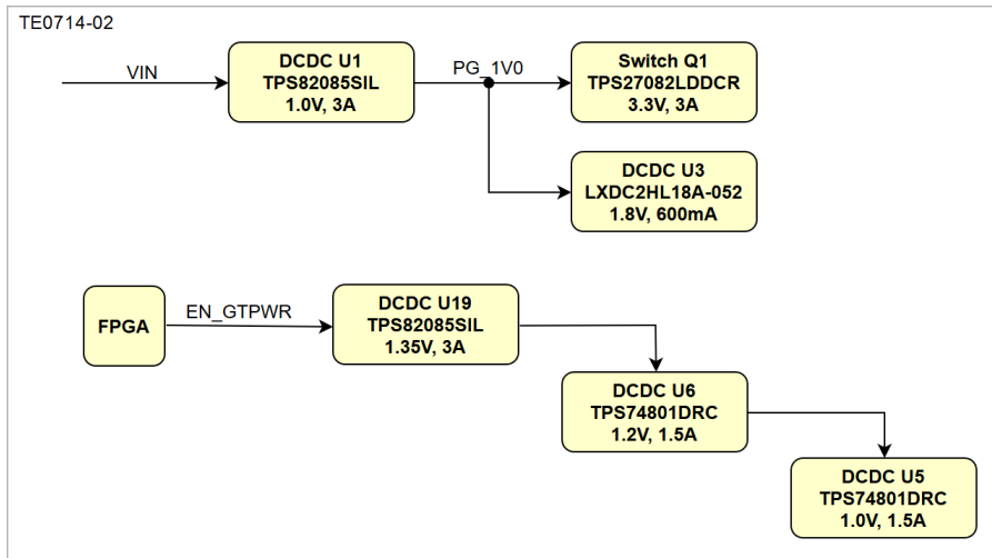
Figure 4: Power-On Sequence
