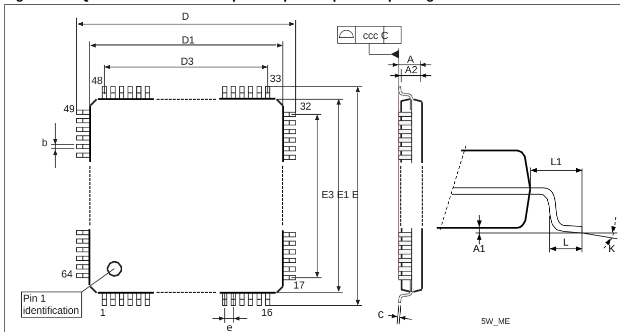
Figure 31. LQFP64 – 10 x 10 mm 64 pin low-profile quad flat package outline
