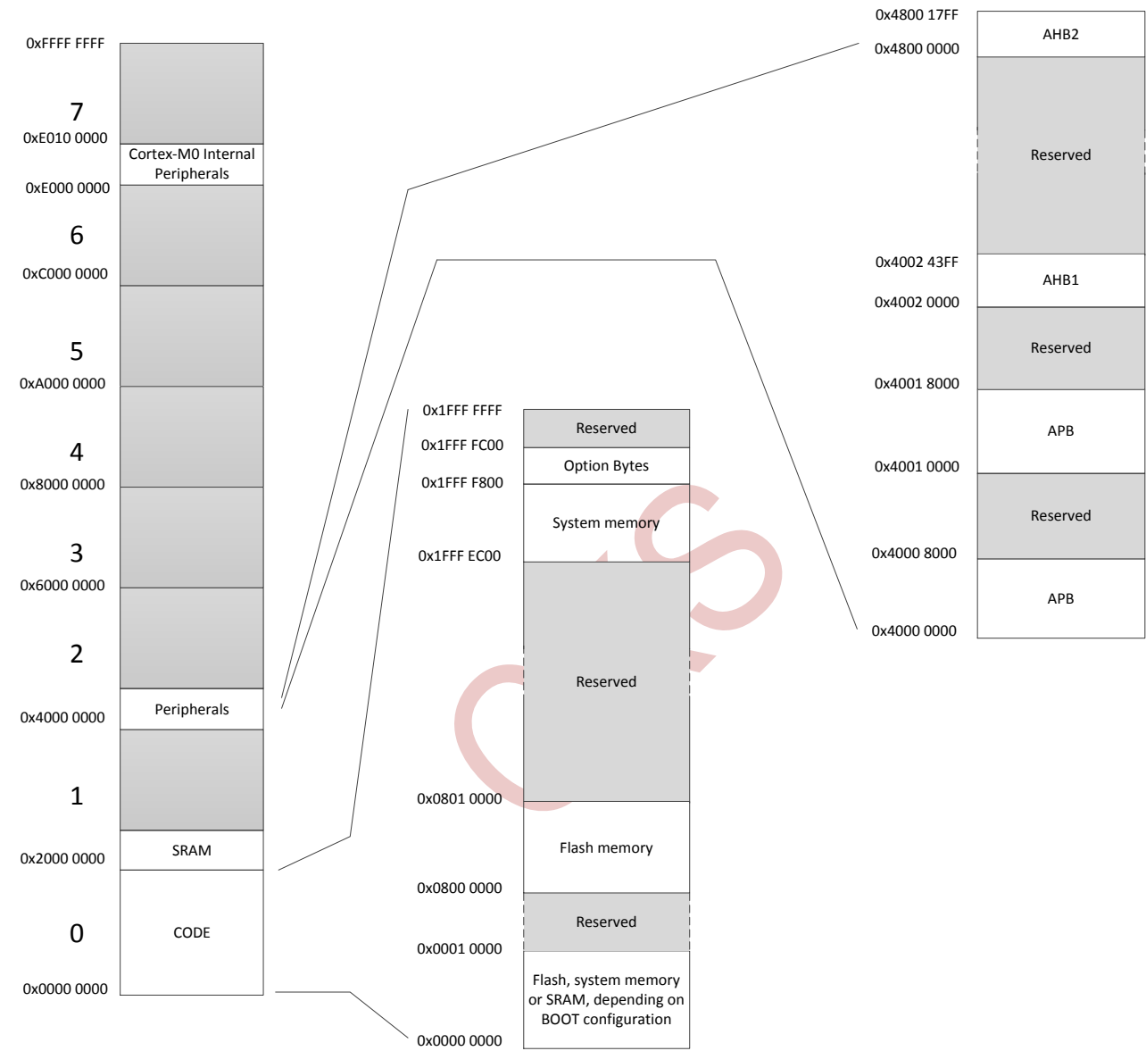
Figure 7. CKS32F051x memory map
