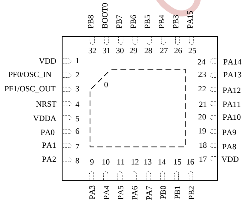
Figure 5. UFQFPN32 32-pin package pinout
