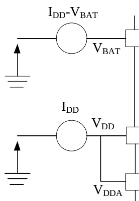
Figure 4. Current consumption measurement scheme
