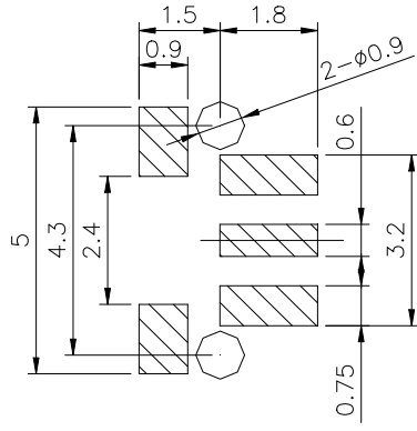
PCB. 焊接图 PCB. WELDING DRAWING
