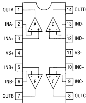
EL2480C (14-Pin SO & 14-Pin PDIP)
