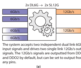
Figure 3-7: Multiplex Conversion Modes
