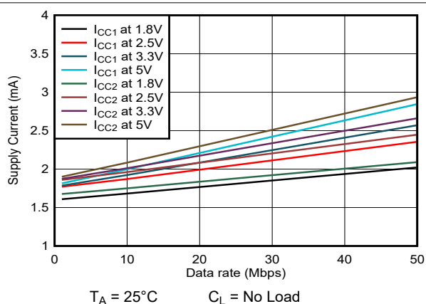
图 5-4. ISO6521 Supply Current vs Data Rate (With No Load)
