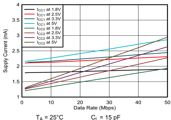
图 5-2. ISO6520 Supply Current vs Data Rate (With No Load)
