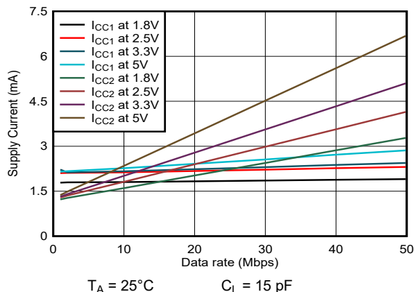
图 5-1. ISO6520 Supply Current vs Data Rate (With 15-pF Load)
