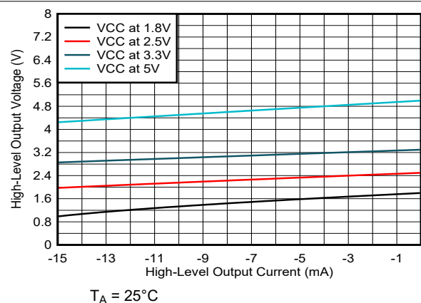
图 5-5. High-Level Output Voltage vs High-level Output Current
