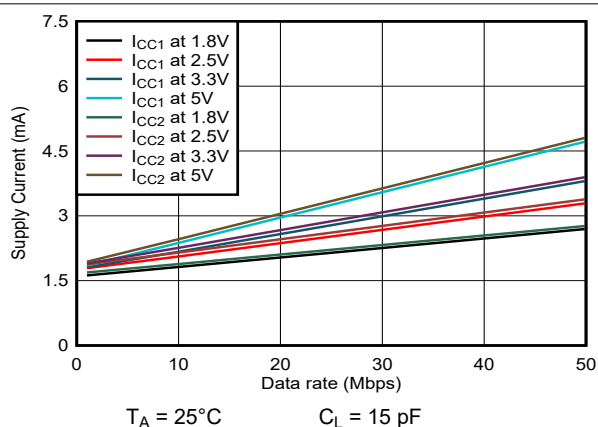
图 5-3. ISO6521 Supply Current vs Data Rate (With 15-pF Load)
