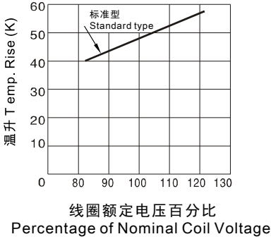
线圈温升 Coil Temperature Rise
