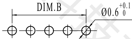
PCB LAYOUT
