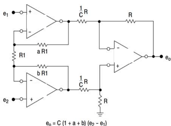
Figure 3. e_o = C (1 + a + b) (e_2 - e_1)
