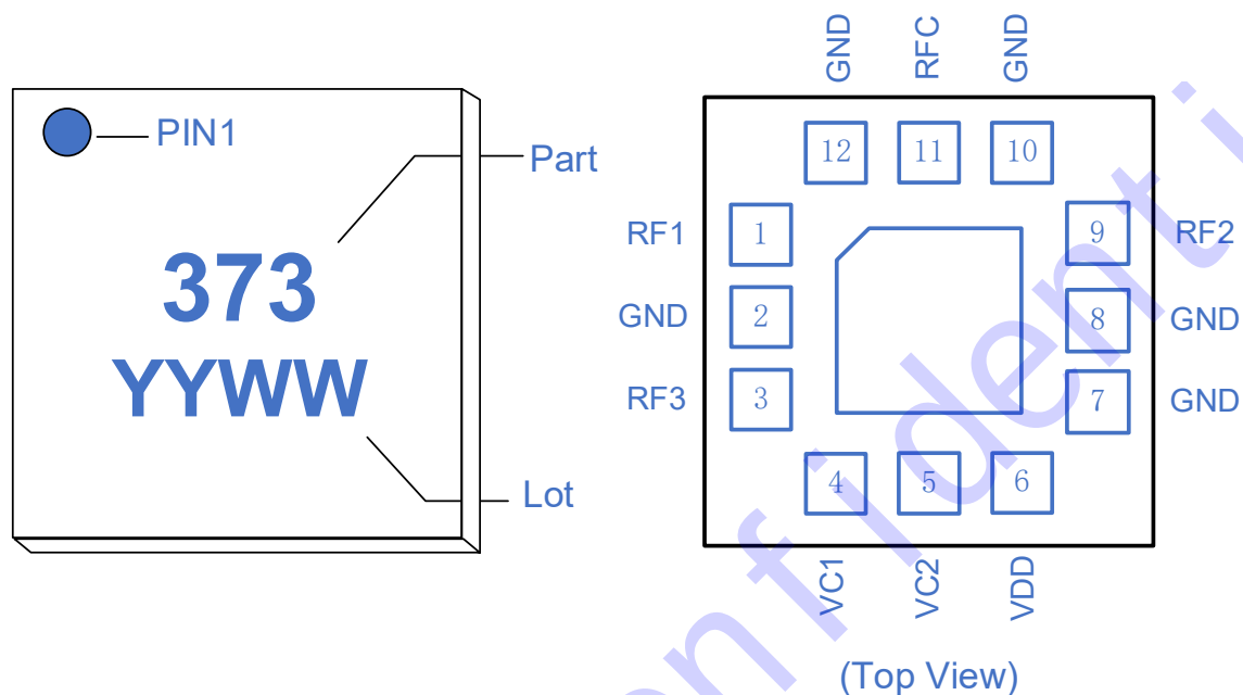
Figure 2 Pin-out Information
