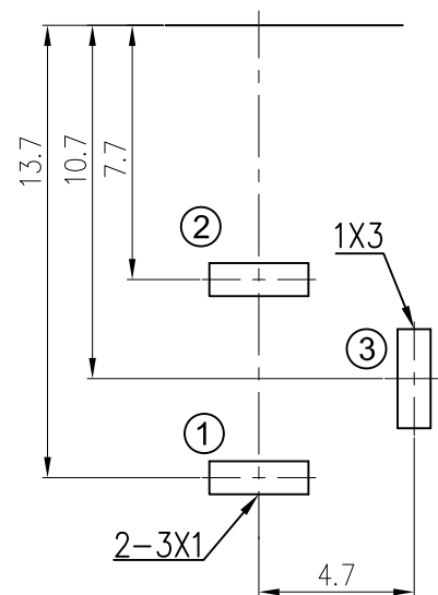
PCB Holes Diagram (VIEWED FROM COPPER SIDE)
