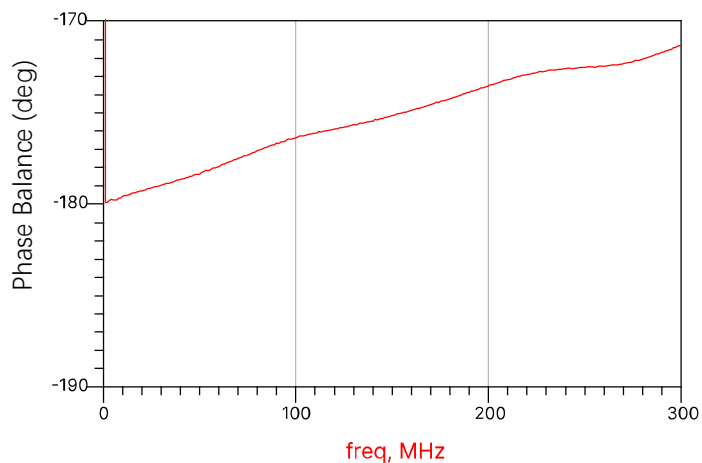
Phase Balance
