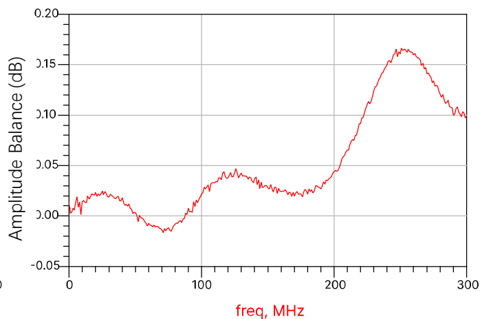
Amplitude Balance
