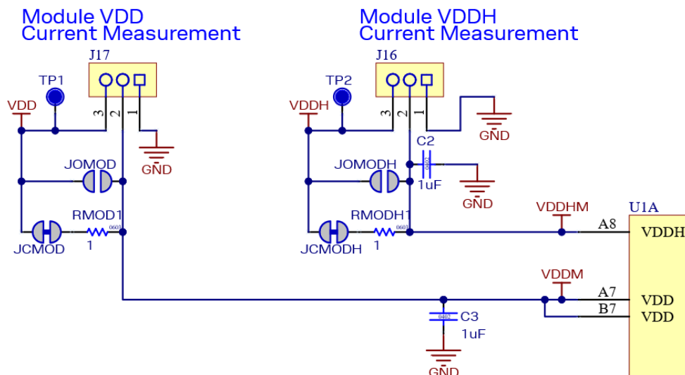
Figure 8: Current measurement
