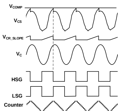
Figure 26: LLC Current Mode Control Waveform
