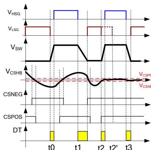
Figure 35: Operating Principle of CMP
