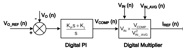
Figure 18: Current Reference
