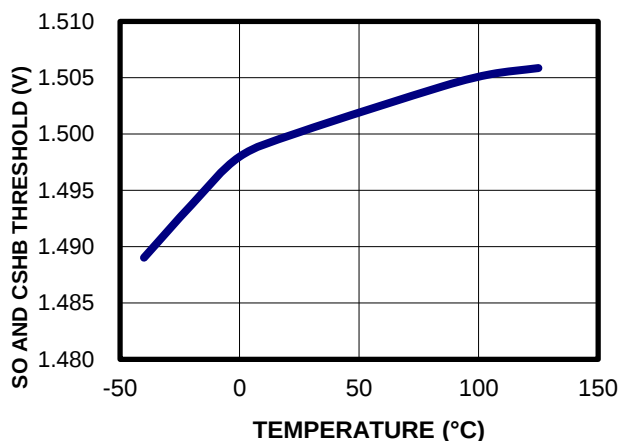
SO and CSHB Threshold vs. Temperature
