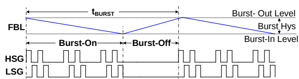
Figure 30: Burst Mode LLC Operation
