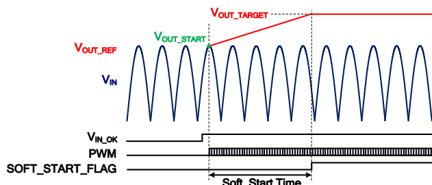
Figure 22: Soft-Start Sequence
