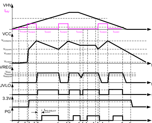
Figure 4: Power Supply Operation Waveform
