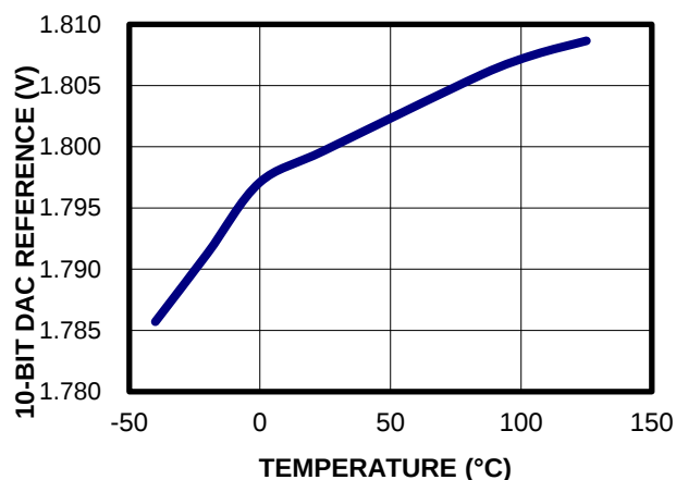
10-Bit DAC Reference vs. Temperature
