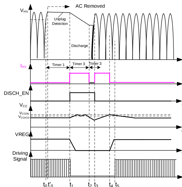
Figure 6: Operating Waveform of the X-Capacitor Discharger when AC Recovers
