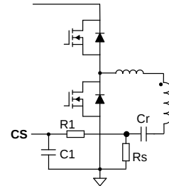
Figure 38: Current Sensing with a Sense Resistor
