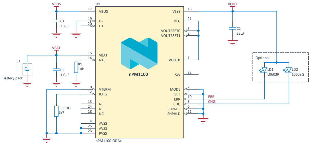
Figure 40: QFN schematic
