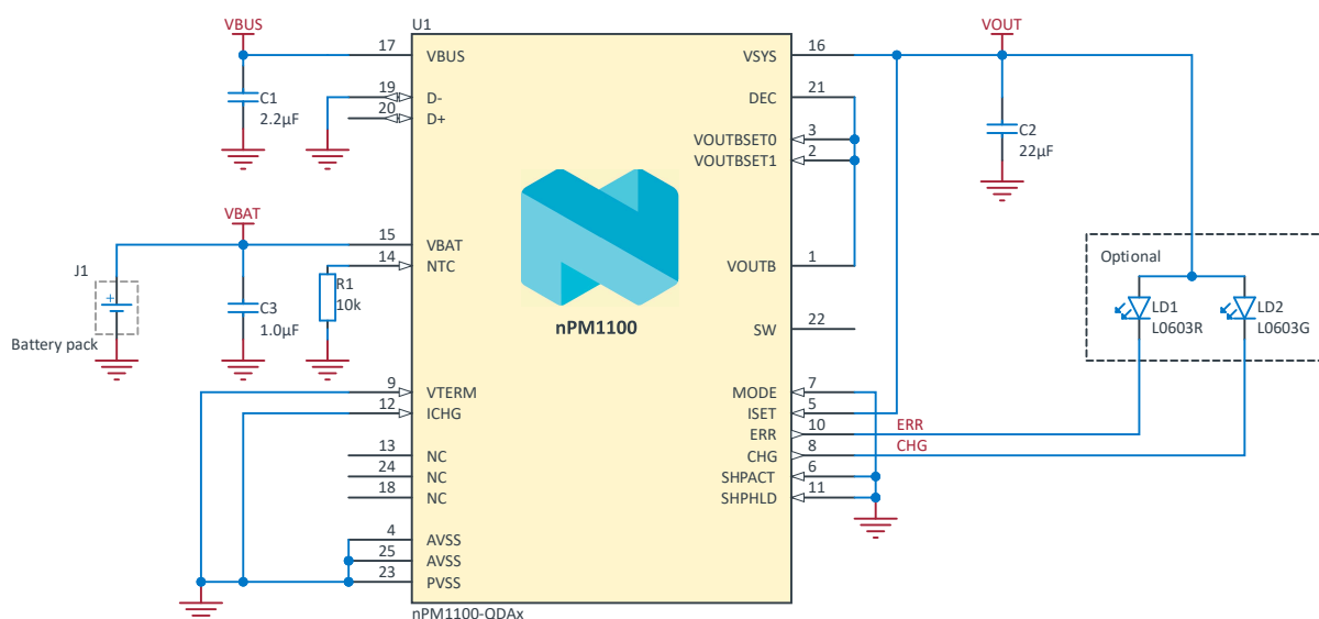
Figure 42: QFN schematic
