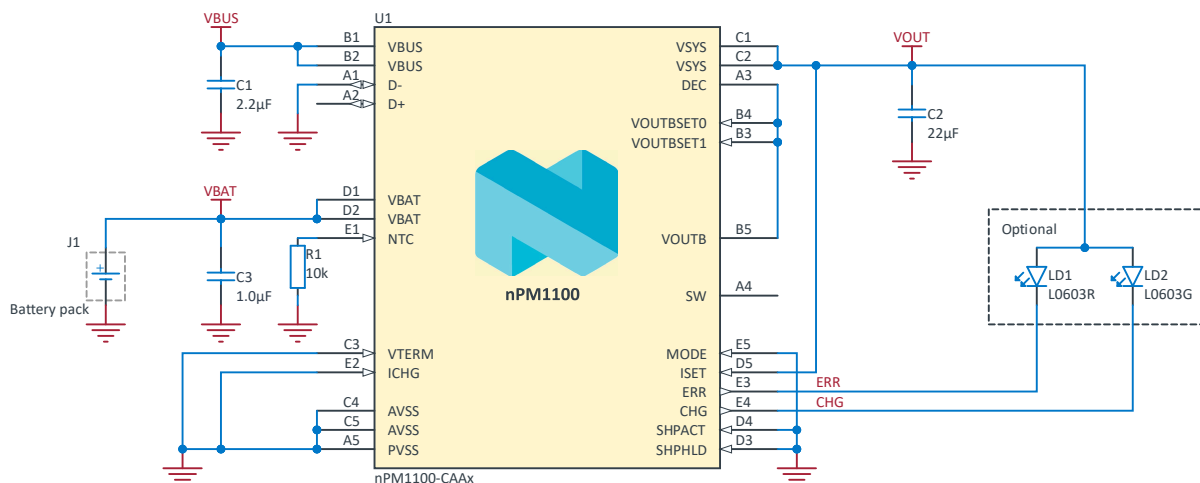
Figure 41: WLCSP schematic
