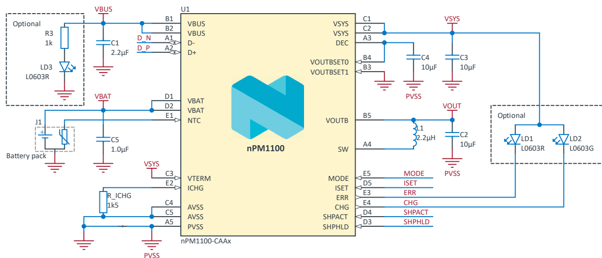
Figure 43: WLCSP schematic
