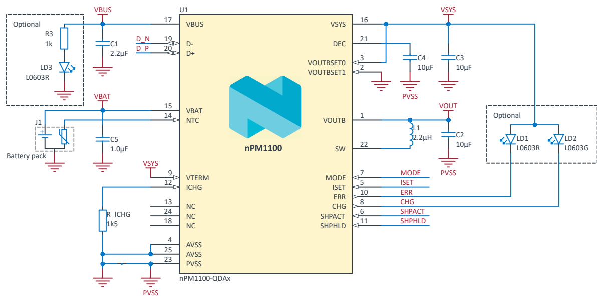
Figure 44: QFN schematic
