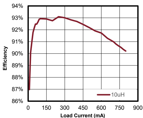
Figure 9.b V_{IN}=4.2\text{V} V_{OUT}=5\text{V}
