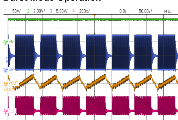
Figure 10.d V_{IN}=5V , V_{OUT(AC)}=12V , LOAD=20mA L=10\mu\text{H} , C_{OUT}=10\mu\text{F} , C_{IN}=4.7\mu\text{F}
