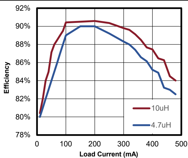
Figure 9.d V_{IN}=5\text{V} V_{OUT}=12\text{V}
