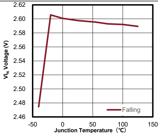
Figure 8.b UVLO Falling vs Temperature
