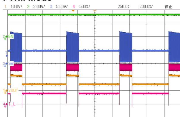
Figure 10.f V_{IN}=5V , V_{OUT}=12V , LOAD=400mA L=10\mu\text{H} , C_{OUT}=10\mu\text{F} , C_{IN}=4.7\mu\text{F}
