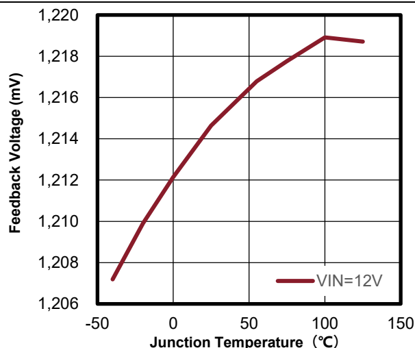
Figure 8.d FB Voltage vs Temperature
