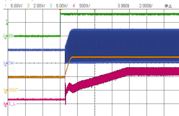
Figure 10.b 5V_{IN} to 12V_{OUT} , LOAD=30R L=10\mu\text{H} , C_{OUT}=10\mu\text{F} , C_{IN}=4.7\mu\text{F}
