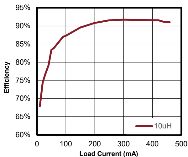
Figure 9.f V_{IN}=12\text{V} V_{OUT}=24\text{V}
