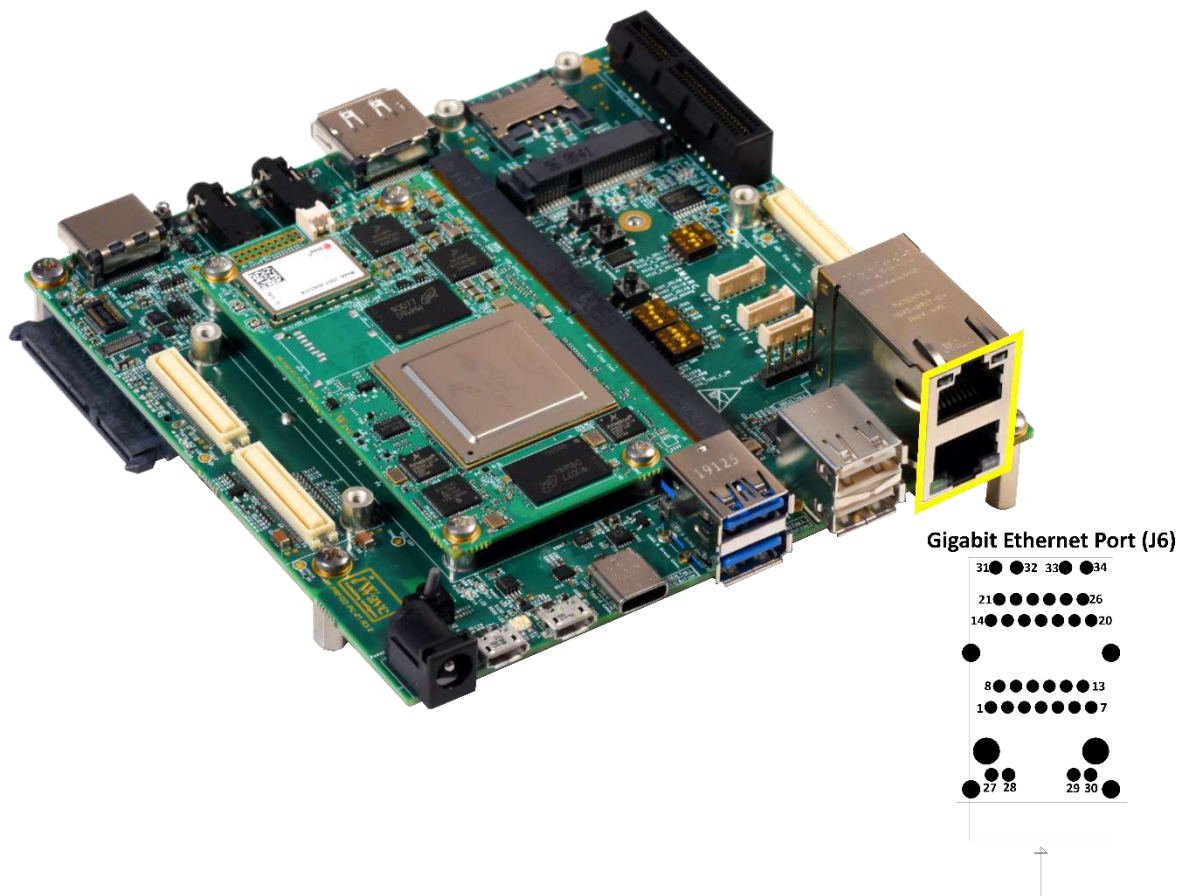
Figure 10: RJ45 Magjack
