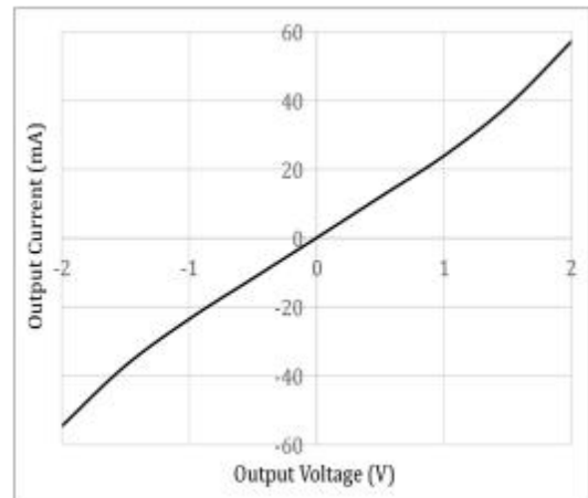
Fig.2 Output Current vs. Output Voltage
