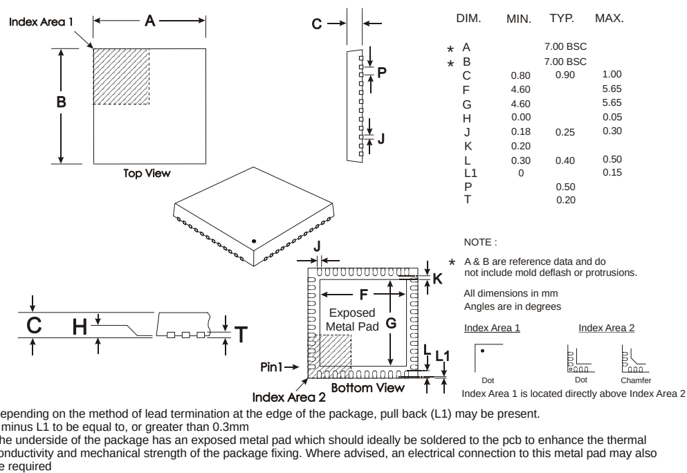
Figure 9 48-pin VQFN Mechanical Outline (Q3) Order as part no. CMX7158Q3
