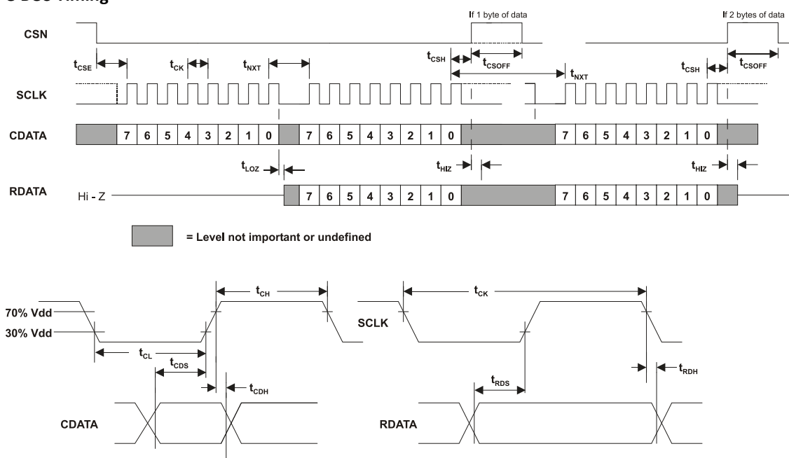
Figure 5 C-BUS Transactions
