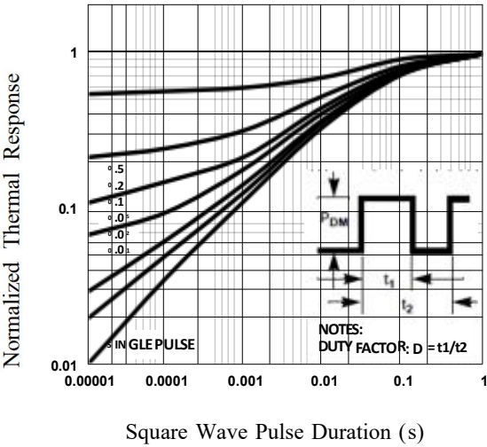
Fig. 9 Normalized Transient
