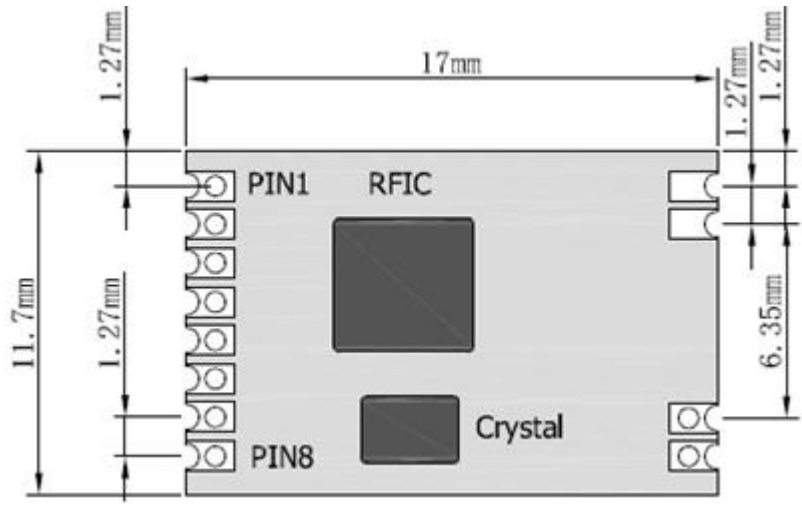
Figure 1: Module size
