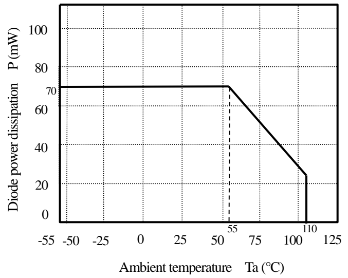
(Fig. 2) Diode power dissipation vs. ambient temperature
