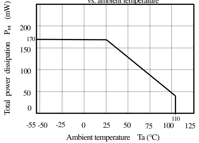
(Fig. 4) Total power dissipation vs. ambient temperature
