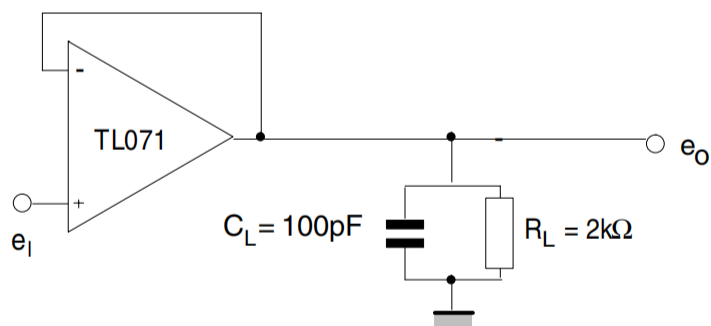
Voltage follower
