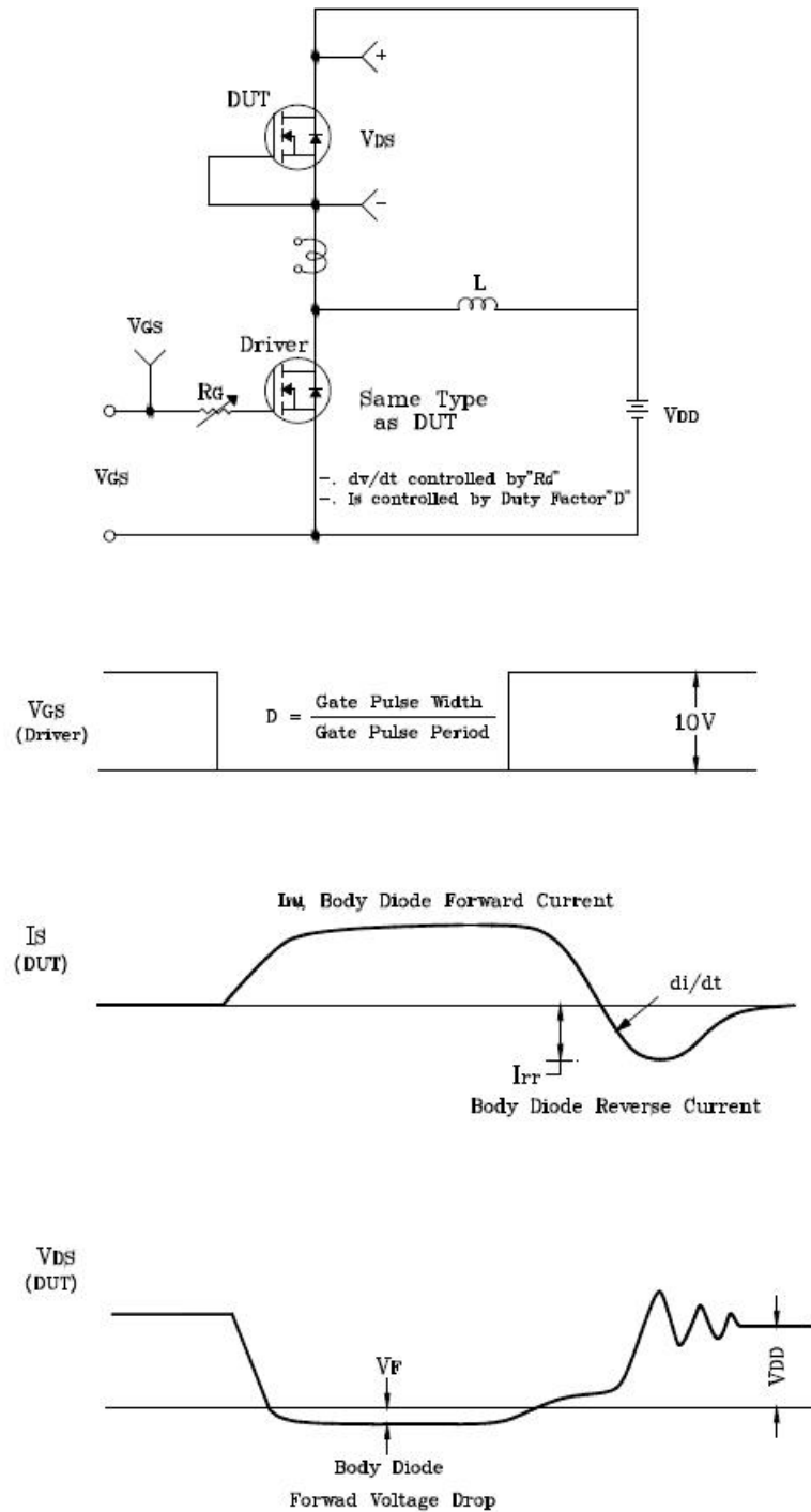
Fig. 15 Diode Reverse Recovery Time Test Circuit & Waveform
