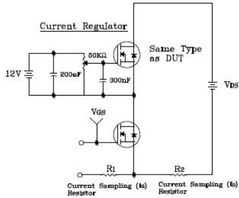
Fig. 12 Gate Charge Test Circuit & Waveform
