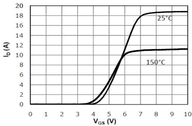
Fig 3: Transfer Characteristics
