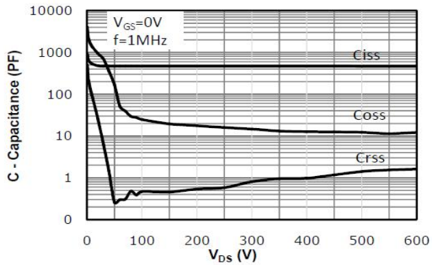
Fig 11: Capacitance Characteristics
