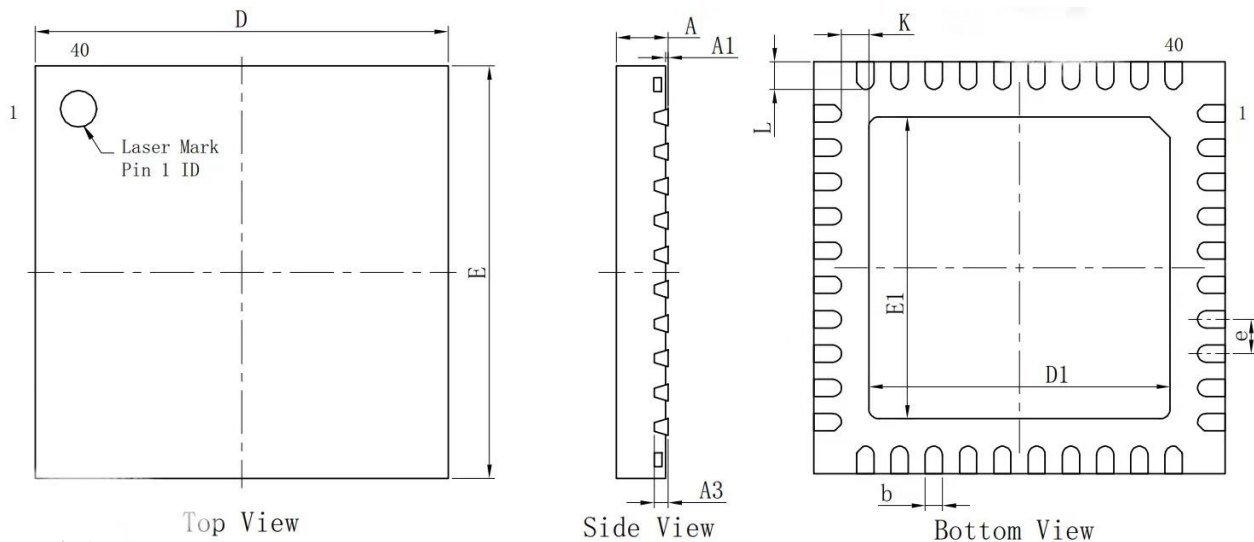
FIGURE 14. QFN-40 PACKAGE OUTLINE DRAWING AND RECOMMENDED PCB LAND PATTERN
