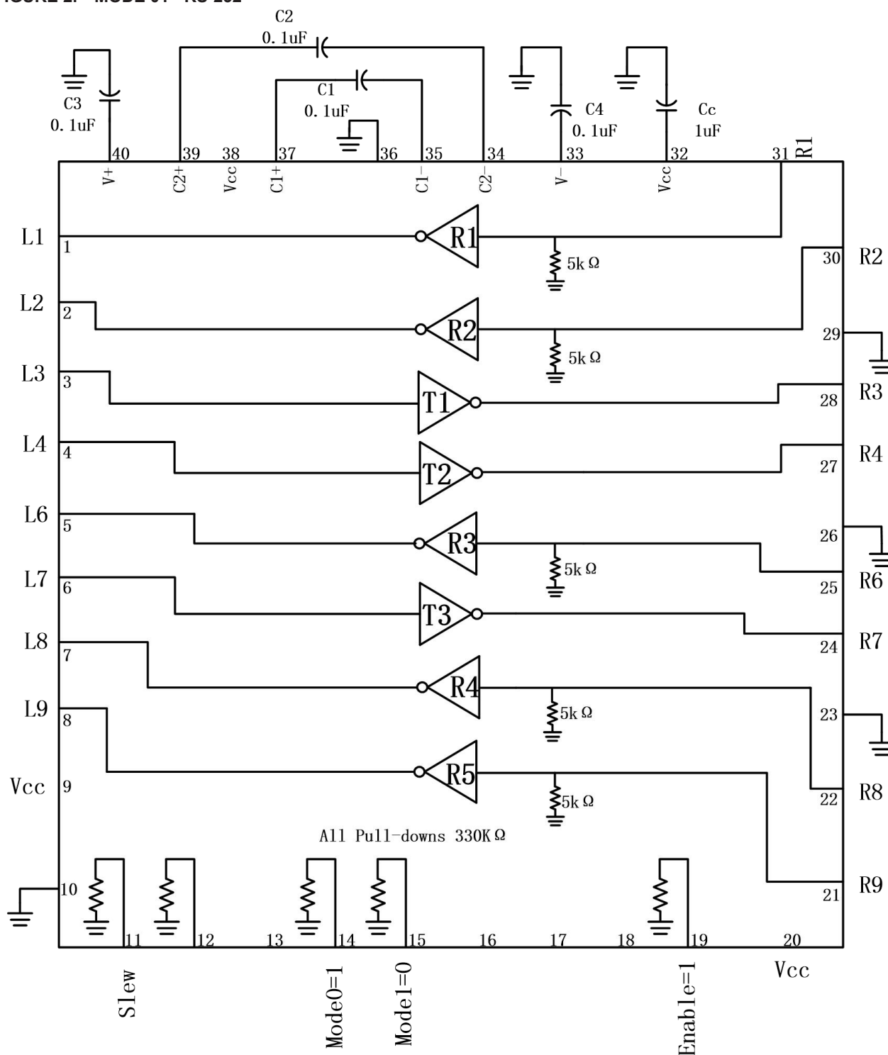
FIGURE 2. MODE 01 - RS-232
